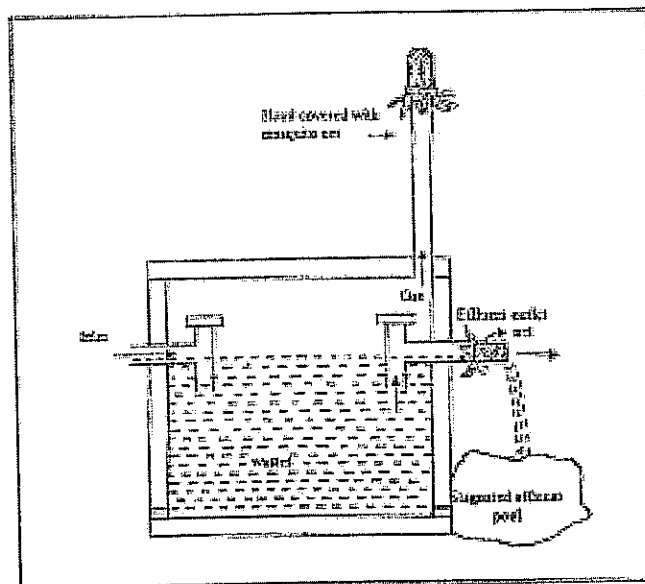
Fig. 1b. Method of controlling mosquito breeding in septic tank
