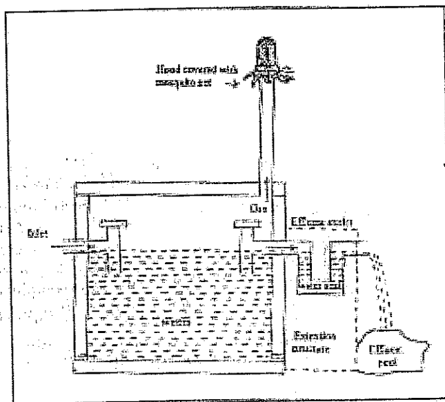
Fig. 1a. Method of controlling mosquito breeding in septic tank
